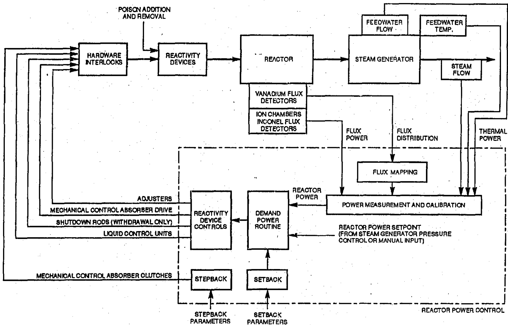
Figure 3.8. Reactor Regulating System-Block Diagram.
